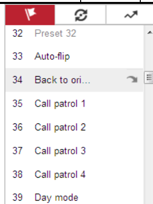
Figure 4-8 Special Preset
