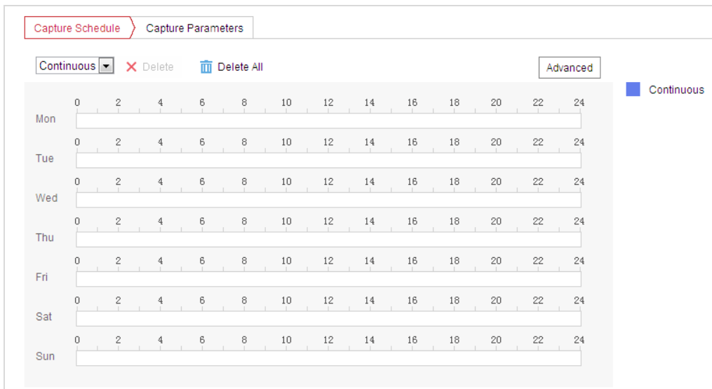
Figure 5-3 Snapshot Settings
