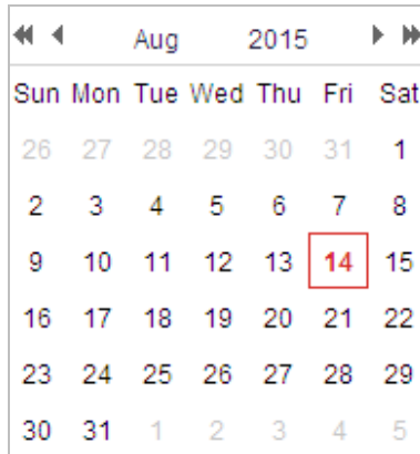
Figure 4-14 Search Video
