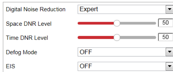
Figure 6-33 Expert Mode
