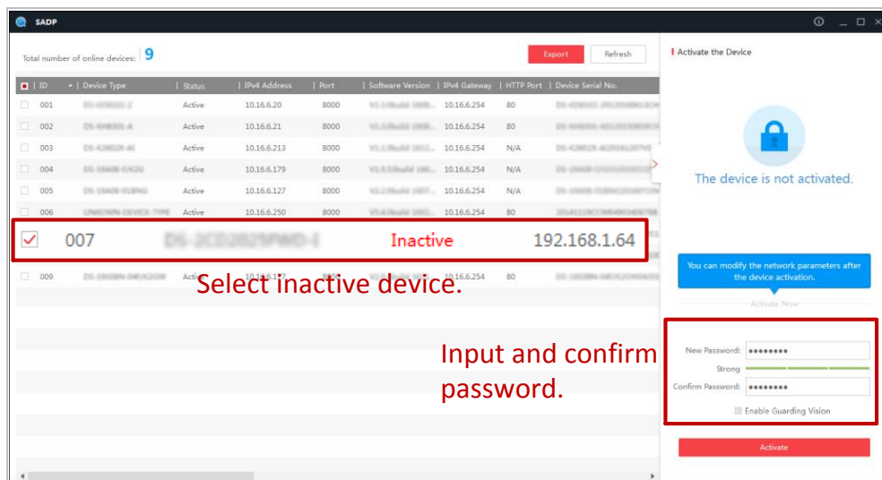
Figure 2-4 SADP Interface
