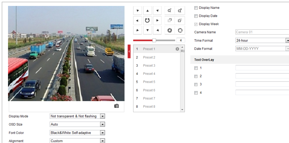
Figure 6-36 OSD Settings
