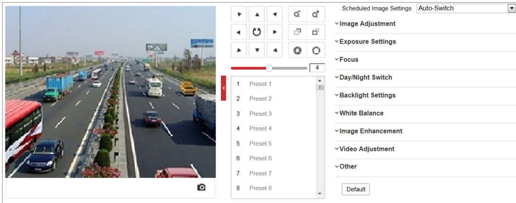
Figure 6-23 Display Settings
